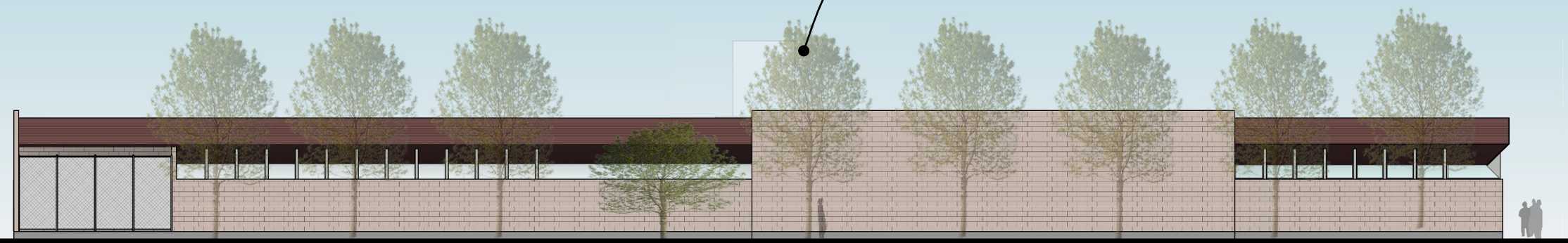
NORTH ELEVATION ARMSTRONG AVENUE
