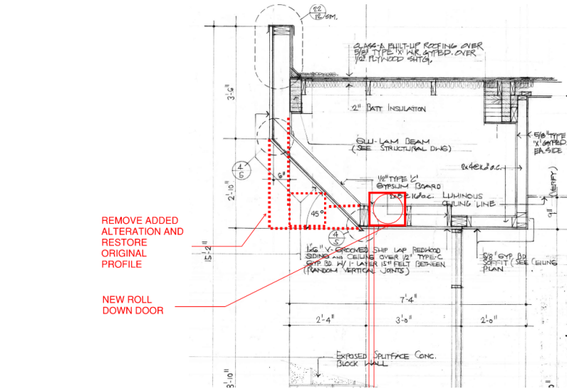
ENTRY FASCIA DETAIL
