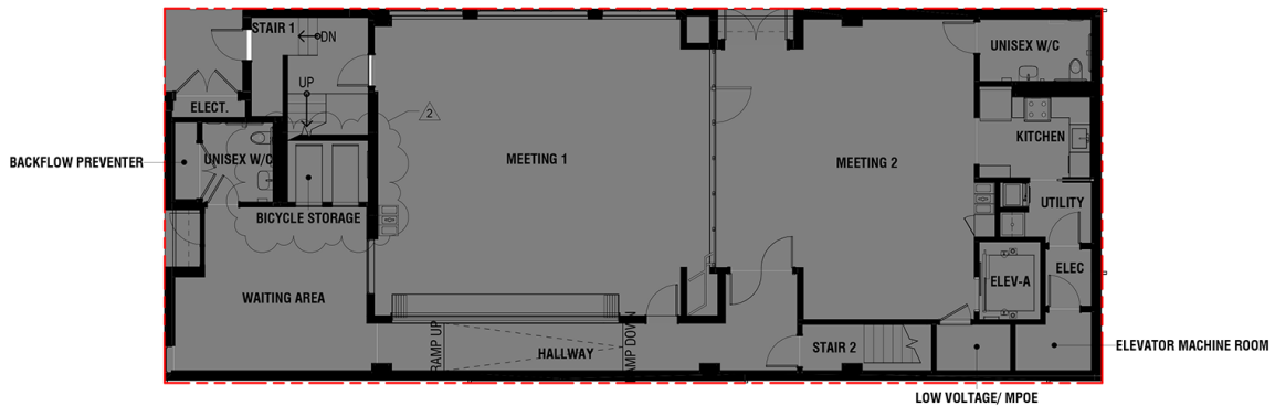
FLOOR PLAN - LEVEL 1 1 SCALE: 1/8" = 1'-0"
