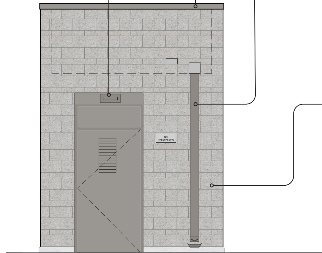
WEST ELEVATION
