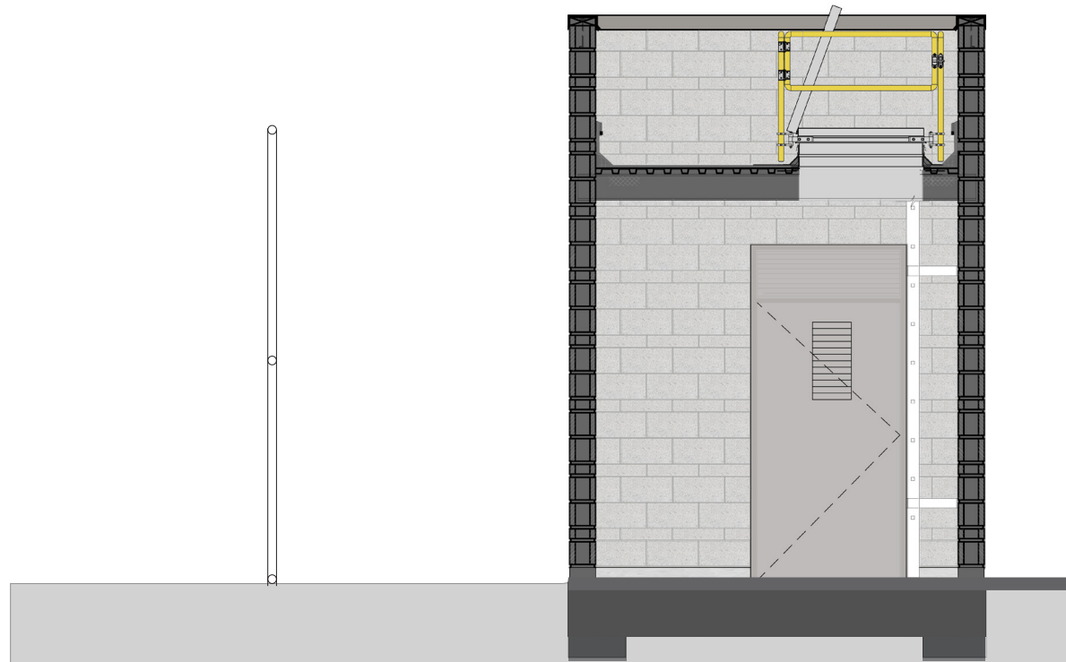
BB - NS SECTION
