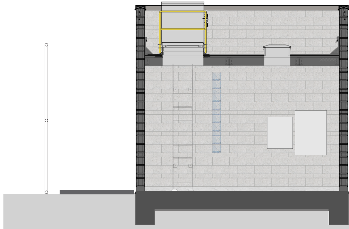
AA - EW SECTION
