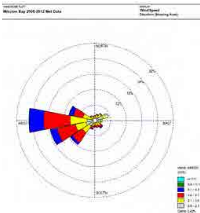
Figure 7. Mission Bay 2008 Wind Rose
